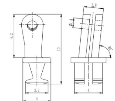
塑铰 Regular hinge for plastic frame
