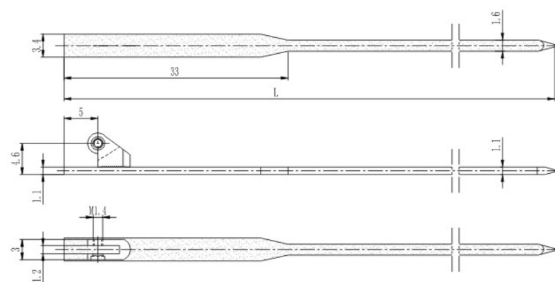
铰链插芯 Regular hinge wire core L136 XHD2080CA1360-YN 材料/Material: 无铅白铜/Lead free nickel silver
