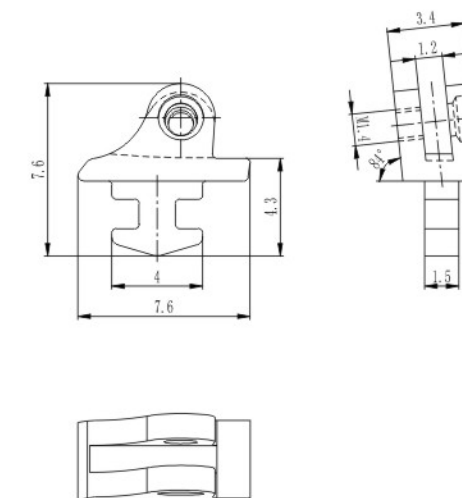
塑铰 Regular hinge for plastic frame XAA4042-34-WN
