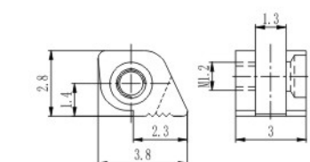
弹簧前铰 Front hinge for metal frame XD7124D30/0
