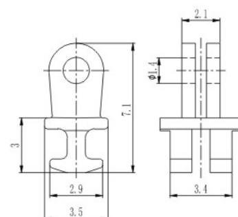
塑铰 Regular hinge for plastic frame XAA4099-45-WN
