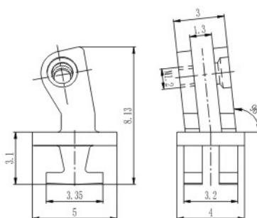
弹簧塑铰 Front hinge for plastic frame XD184-C40/WG01
