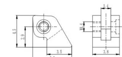
弹簧前铰 Front hinge for metal frame XD754-38/0
