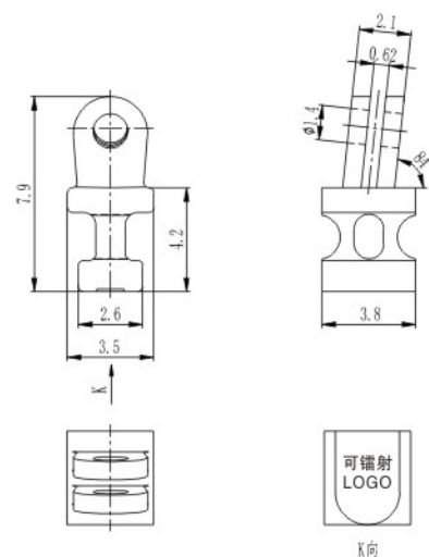
塑铰 Regular hinge for plastic frame XAA4053-38-WN 材料/Material: 无铅白铜/Lead free nickel silver
