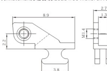
弹簧塑铰 Front hinge for plastic frame XD854-27/N0
