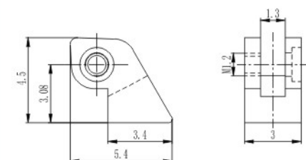
弹簧前铰 Front hinge for metal frame XD7030-30/0
