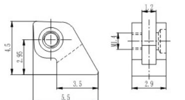
弹簧前铰 Front hinge for metal frame XD754-29/0
