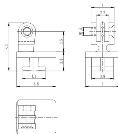
塑铰 Regular hinge for plastic frame XAA4060-60-WN 材料/Material: 无铅白铜/Lead free nickel silver
