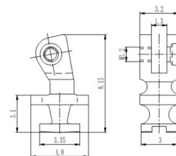
弹簧塑铰 Front hinge for plastic frame XDB184-32-WN
