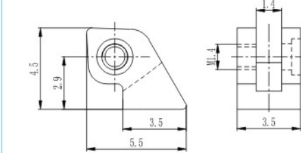
弹簧前铰 Front hinge for metal frame XD754-35/0
