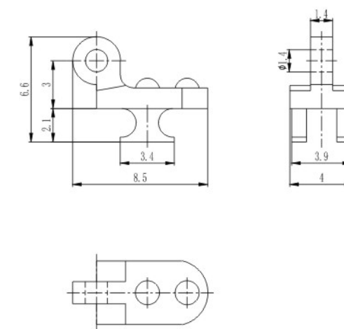
塑铰 Regular hinge for plastic frame XAA4149-40-WN 材料/Material: 无铅白铜/Lead free nickel silver
