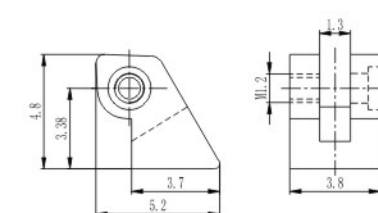
弹簧前铰 Front hinge for metal frame XD014-38/0
