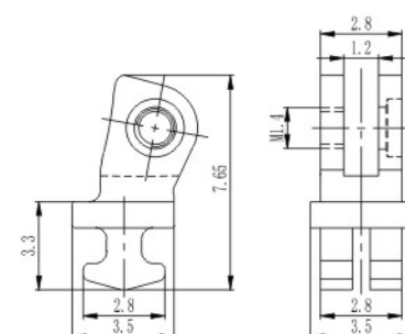
弹簧塑铰 Front hinge for plastic frame
