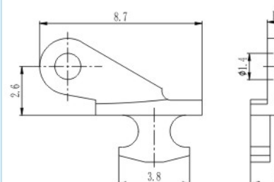
塑铰 Regular hinge for plastic frame XA071-A30/WG01 材料/Material: 无铅白铜/Lead free nickel silver
