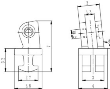
弹簧塑铰 Front hinge for plastic frame XD7014-40/N0
