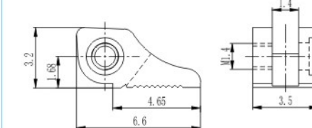
弹簧前铰 Front hinge for metal frame XD706-35/0
