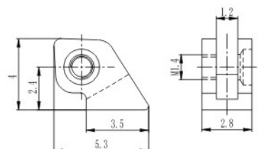
弹簧前铰 Front hinge for metal frame XD7046-28/0
