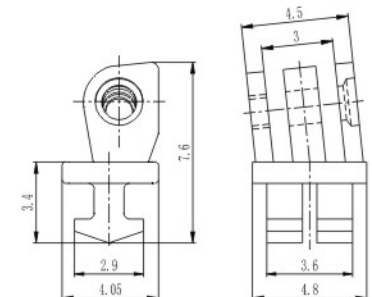
弹簧塑铰 Front hinge for plastic frame
