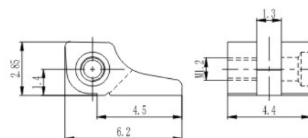
弹簧前铰 Front hinge for metal frame
