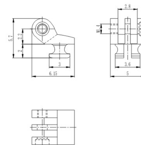
塑铰 Regular hinge for plastic frame XAA3008-50-WN 材料/Material: 无铅白铜/Lead free nickel silver
