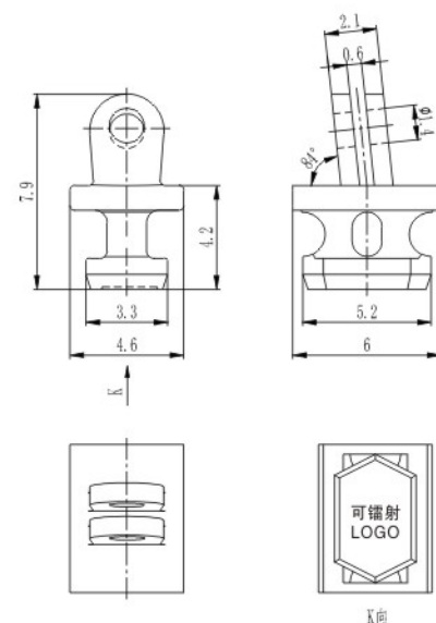
塑铰 Regular hinge for plastic frame XAA4071A60-WN 材料/Material: 无铅白铜/Lead free nickel silver
