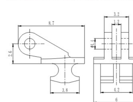
塑铰 Regular hinge for plastic frame
