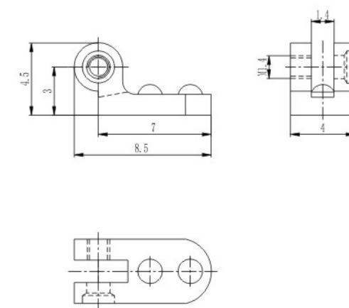
塑铰 Regular hinge for plastic frame XAE4178-40-W 材料/Material: 无铅白铜/Lead free nickel silver
