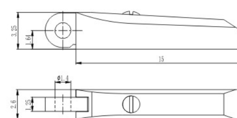
组合弹簧盒 Spring hinge XFP939B26/Y
