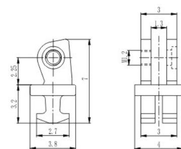
弹簧塑铰 Front hinge for plastic frame XD7014M40/N0
