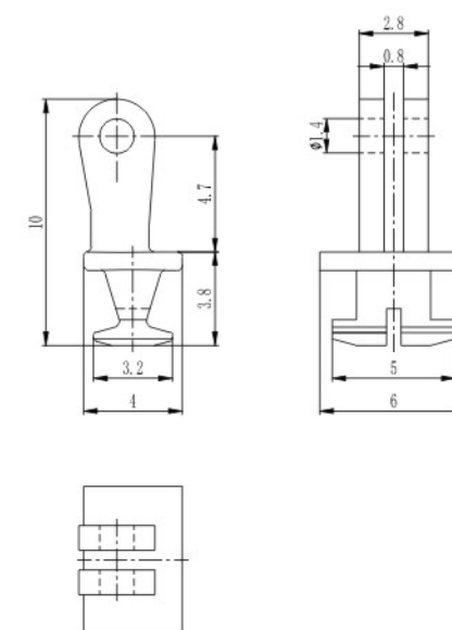
塑铰 Regular hinge for plastic frame XA3069-D60/WG01
