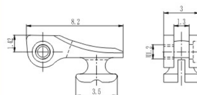
弹簧塑铰 Front hinge for plastic frame XD798-30/N0
