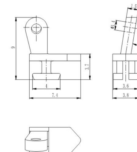
塑铰 Regular hinge for plastic frame XAA4049-38-WN
