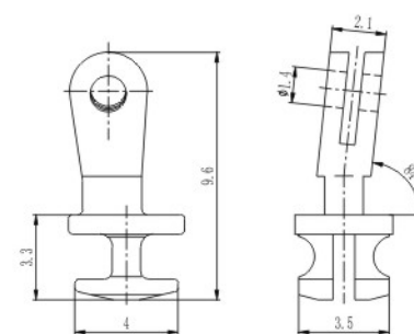
塑铰 Regular hinge for plastic frame XAA3169B38-WN
