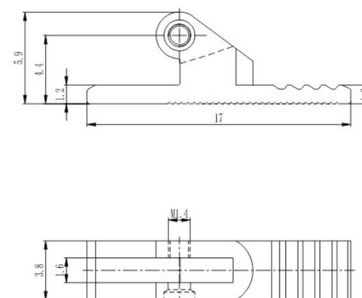
注塑铰链 Injection hinge
