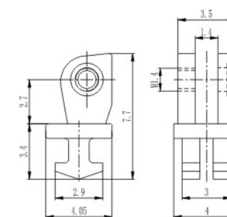
弹簧塑铰 Front hinge for plastic frame XD734E40/N0
