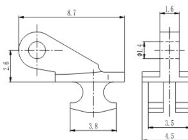
塑铰 Regular hinge for plastic hinge XA071-45/NO
