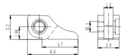
弹簧前铰 Front hinge for metal frame XD706C28/0
