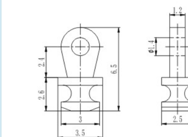
塑铰 Regular hinge for plastic frame XA3013-25/N0 材料/Material: 无铅白铜/Lead free nickel silver
