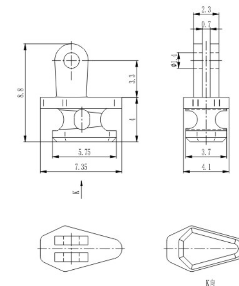
塑铰 Regular hinge for plastic frame XAA4135-41-WP2 材料/Material: 无铅白铜/Lead free nickel silver
