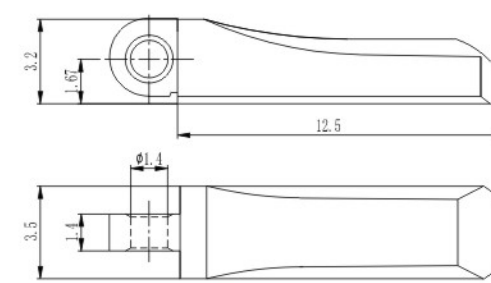
组合弹簧盒 Spring hinge XFP7025-35/0
