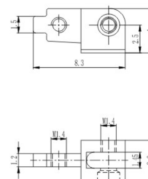
庄头 Lug XCA4214-36-WN 材料/Material: 无铅白铜/Lead free nickel silver
