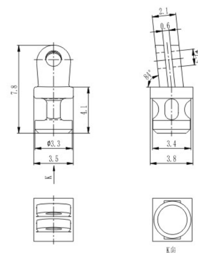
塑铰 Regular hinge for plastic frame XAA4091E38-WN 材料/Material: 无铅白铜/Lead free nickel silver
