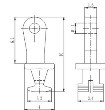
塑铰 Regular hinge for plastic frame XA3069-A40/WG01
