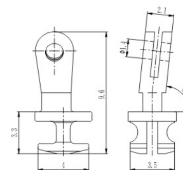
塑铰 Regular hinge for plastic frame XAA3169B38-WN
