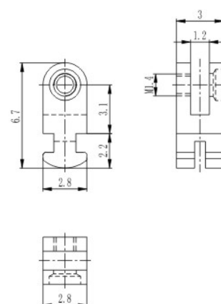
塑铰 Regular hinge for plastic frame XA3064-30/WG01
