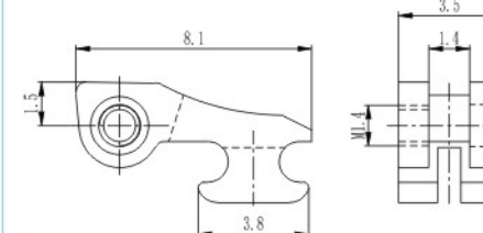
弹簧塑铰 Front hinge for plastic frame XD774-35/N0
