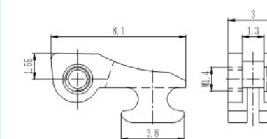
弹簧塑铰 Front hinge for plastic frame XDB8516-30-WN
