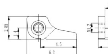
弹簧前铰 Front hinge for metal frame XD7134-30/0
