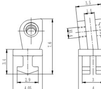
弹簧塑铰 Front hinge for plastic frame XD734-40/N0
