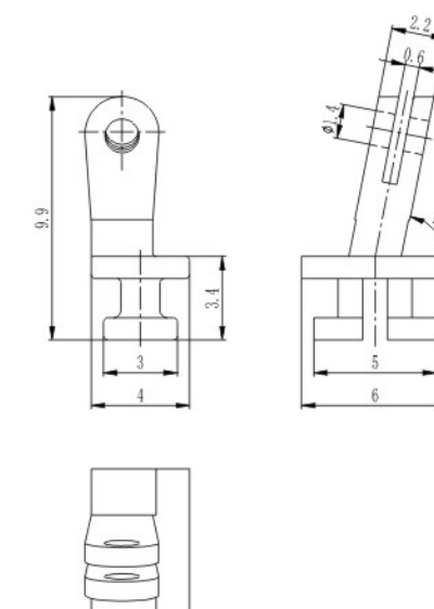
塑铰 Regular hinge for plastic frame XAA4047A60-WN
