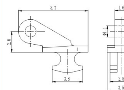
塑铰 Regular hinge for plastic frame XA071-35/N0 材料/Material: 无铅白铜/Lead free nickel silver
