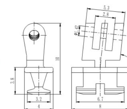
对口铰 Regular hinge for metal frame XBA1296A80-W 材料/Material: 无铅白铜/Lead free nickel silver
