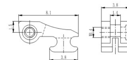
弹簧塑铰 Front hinge for plastic frame XD774-38/N0
