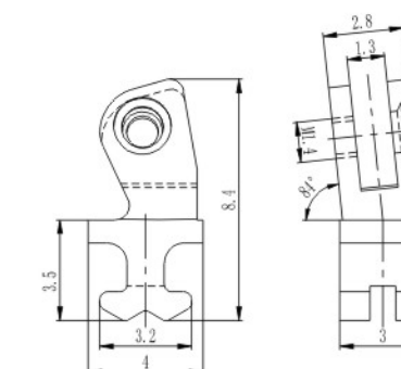
弹簧塑铰 Front hinge for plastic frame
