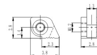
弹簧前铰 Front hinge for metal frame XDA7124A28-W
