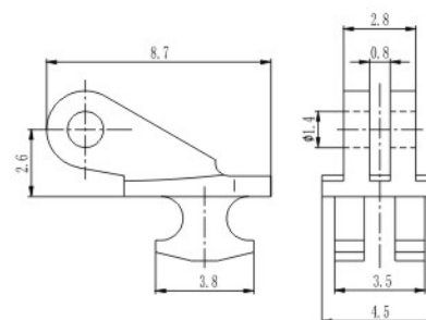
塑铰 Regular hinge for plastic frame
