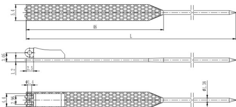
弹簧插芯 Spring hinge wire core
