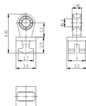
加胶铰链 Safely hinge XAD023C35-WN
