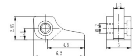
弹簧前铰 Front hinge for metal frame XD7134-30/0
