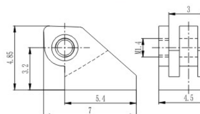
弹簧前铰 Front hinge for metal frame
