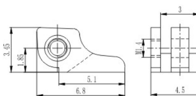
弹簧前铰 Front hinge for metal frame
