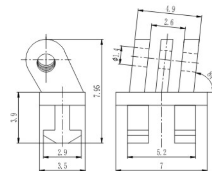
对口铰 Regular hinge for metal frame XB170-A70/W 材料/Material: 无铅白铜/Lead free nickel silver
