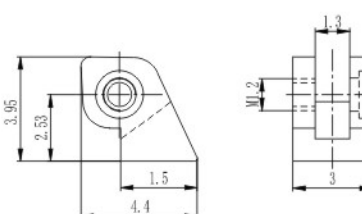
弹簧前铰 Front hinge for metal frame XD7032A30/0
