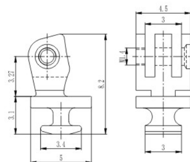
弹簧塑铰 Front hinge for plastic frame
