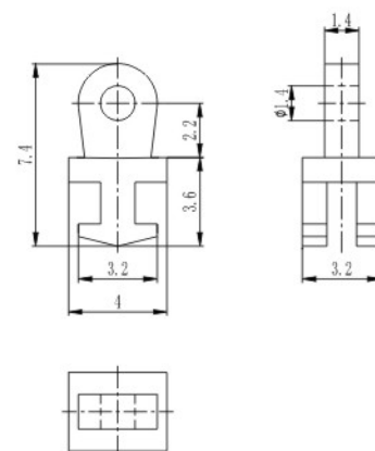
塑铰 Regular hinge for plastic frame XA119-32/N0 材料/Material: 无铅白铜/Lead free nickel silver
