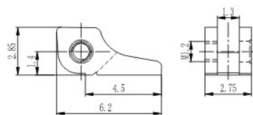
弹簧前铰 Front hinge for metal frame XD7134-27/0
