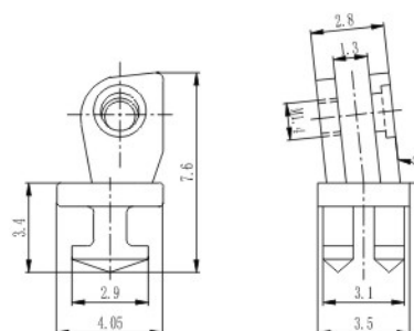
弹簧塑铰 Front hinge for plastic frame XD928H35/N0
