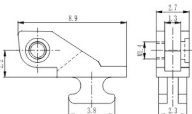
弹簧塑铰 Front hinge for plastic frame XD854-27/N0
