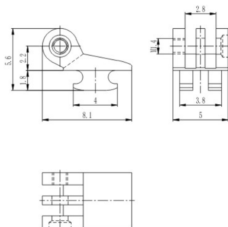
塑铰 Regular hinge for plastic frame XAA4028-50-WN 材料/Material: 无铅白铜/Lead free nickel silver
