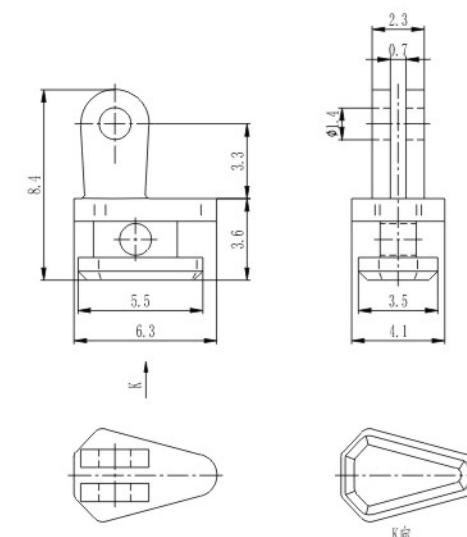
塑铰 Regular hinge for plastic frame XAA4105-41-WM2 材料/Material: 无铅白铜/Lead free nickel silver
