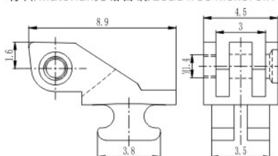
弹簧塑铰 Front hinge for plastic frame
