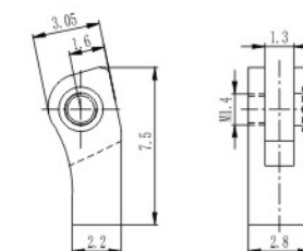
弹簧前铰 Front hinge for metal frame XD054-28/0
