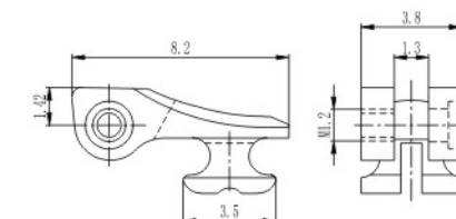
弹簧塑铰 Front hinge for plastic frame XD798B38/N0
