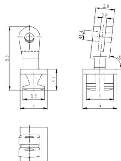
塑铰 Regular hinge for plastic frame XAA4037-50-WN 材料/Material: 无铅白铜/Lead free nickel silver
