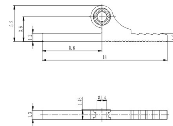
加胶注塑铰链 Safely injection hinge
