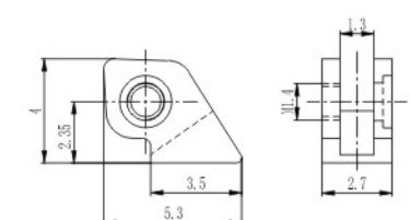
弹簧前铰 Front hinge for metal frame XD8502-F27/0
