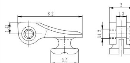
弹簧塑铰 Front hinge for plastic frame XD798-30/N0
