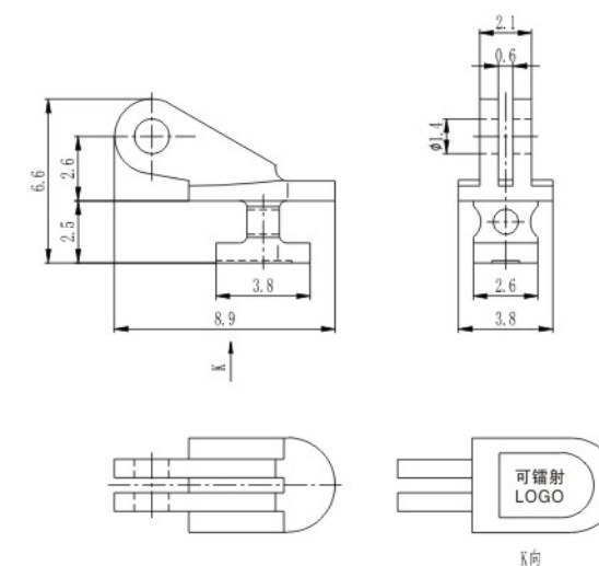
塑铰 Regular hinge for plastic frame XAA4113-38-WN 材料/Material: 无铅白铜/Lead free nickel silver
