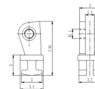
弹簧塑铰 Front hinge for plastic frame XD224-35/WG01
