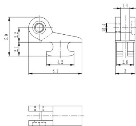
塑铰 Regular hinge for plastic frame XA2610C30/N0 材料/Material: 无铅白铜/Lead free nickel silver
